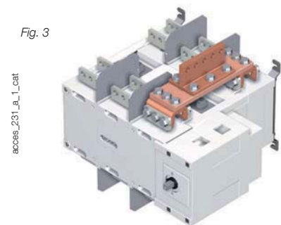
Top or bottom bridging connection
